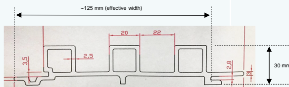
DETAILED DIMENSIONS
